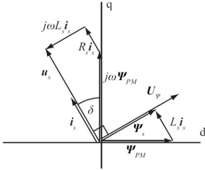
Fig. 11. Phasor diagram for the MegaNdrive sensorless control (not drawn to scale).
