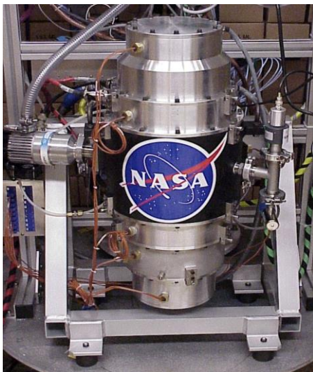
Fig. 7. NASA G2 flywheel for attitude control and energy storage (night-day). 40 000 rpm, 3 kW motor/generator [26].
