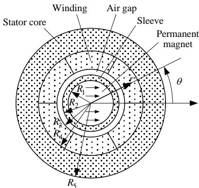
Fig. 8. Machine cross-section: diametrically magnetized cylindrical permanent magnet rotor inside a slotless stator.
