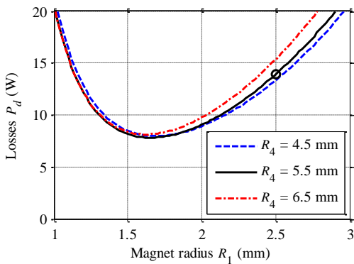
Fig. 9. Losses of a machine with fixed outer dimensions of the stator core ( R_5 = 8 mm, L = 15 mm) and a shaft power of 100 W at a rotational speed of 500 000 rpm for variable magnet radius R_1 . The circle shows the value for the traditional design [34].
