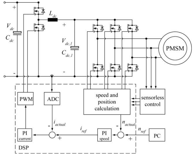
Fig. 10. Power electronics and control system for driving an ultra-high-speed permanent-magnet machine ( MegaNdrive ).
