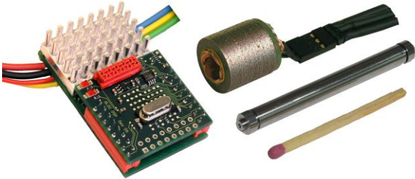
Fig. 14. 100 W, 500 000 rpm drive system including electronics, stator and test bench rotor (two magnets: motor and generator).
