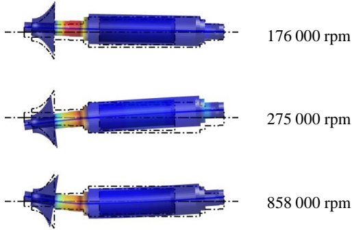
Fig. 13. Bending modes of the Solar Impulse turbocompressor rotor. The color indicates the area of highest mechanical stresses.
