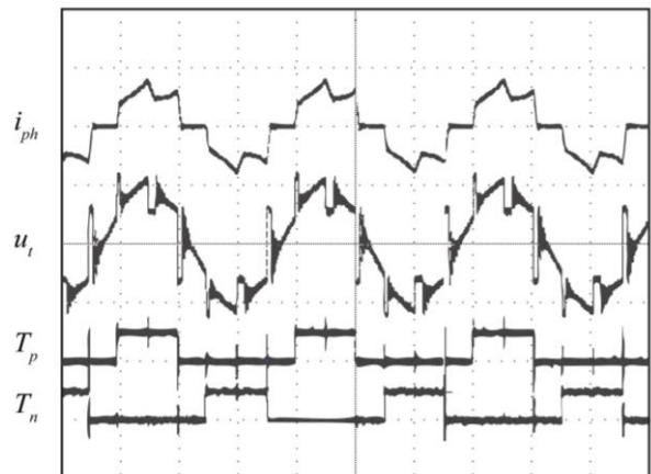
Fig. 17. Measurement (20 \mu s/div) of motor phase current i_{ph} (5 A/div), terminal phase voltage u_t (25 V/div) and half bridge switching signals T_p and T_n at 1 000 000 rpm no load operation.
