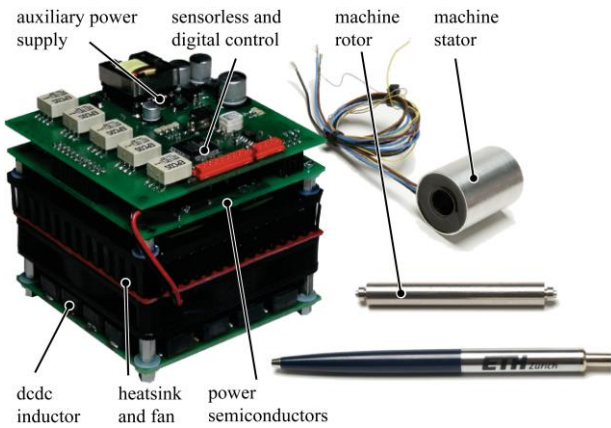
Fig. 15. Power and control electronics, stator and rotor of the 1 kW, 500 000 rpm gas turbine starter/generator.
